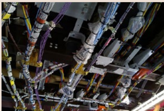
AmberStrand® lightweight composite metal-clad microfilament braid is Glenair's lightest weight material for EMI/RFI shielding applications
