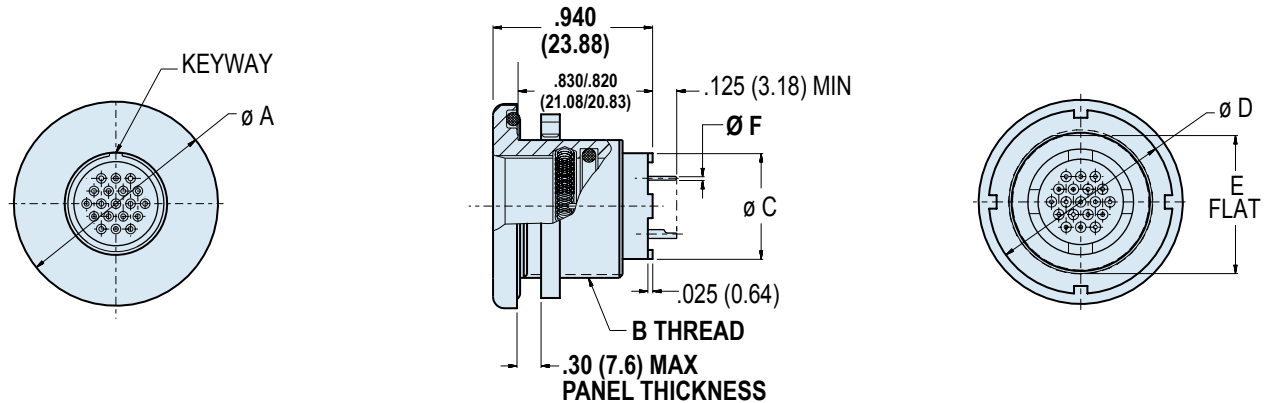
Front Panel Jam Nut 804-006-00
