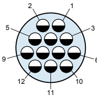
Insert Arrangement 14-12, 16-12, 18-12 12 #16 Contacts .064 (1.63) Max Dia. Tail
