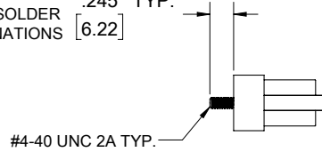
A THREADED STUD COMPATIBLE W/ HARDWARE 0, A, B, T
