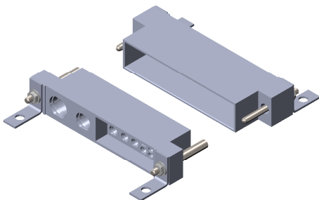
W & X RIGHT ANGLE BRACKET COMPATIBLE W/ HARDWARE STYLE 0, A, B, H, K, T
